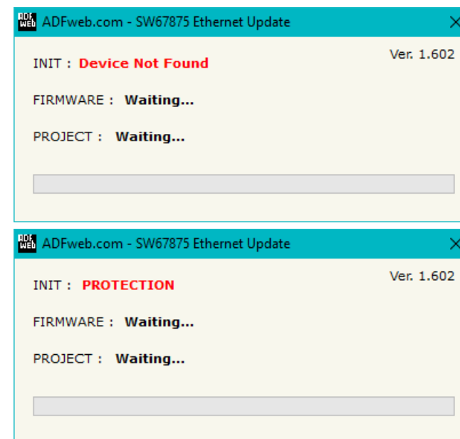
Figure 16: "Error" window
