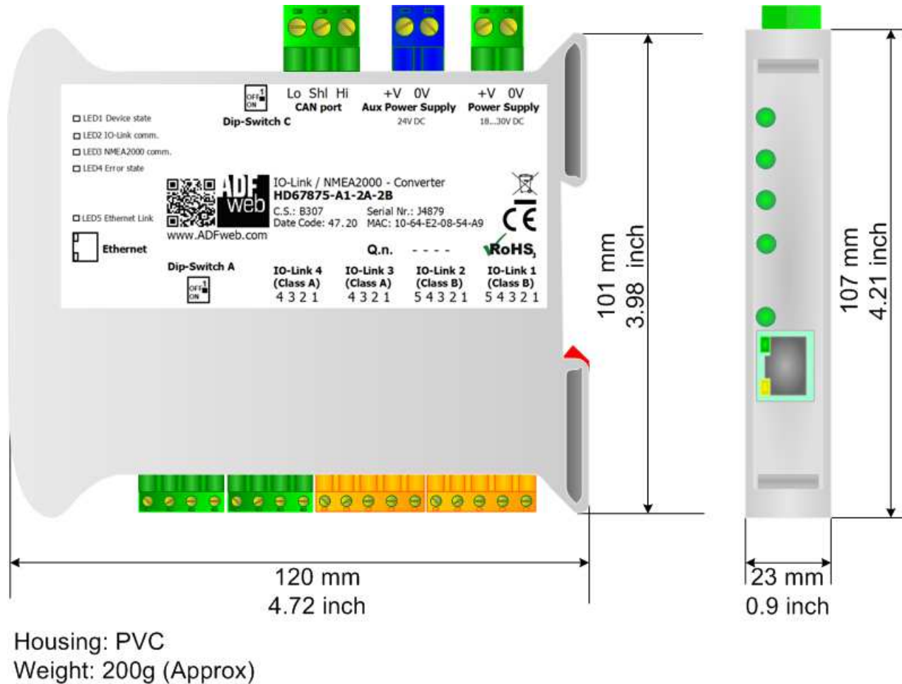
Figure 17: Mechanical dimensions scheme for HD67875-A1-xx
