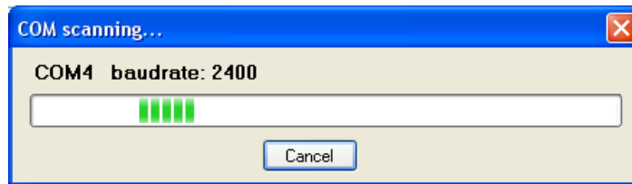
Figure 7: : Automatic search
