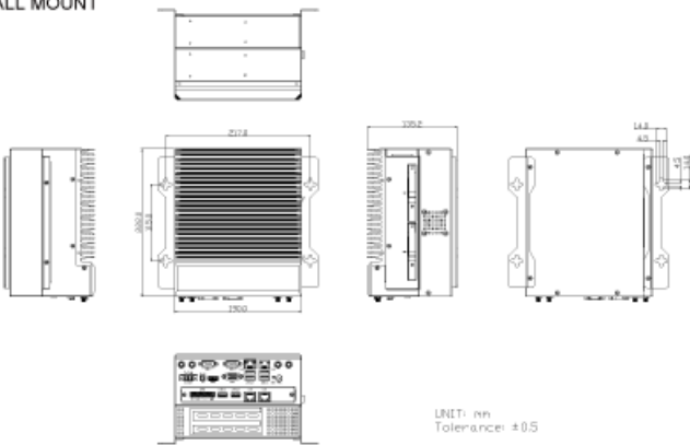
AVS-522 WALL MOUNT
